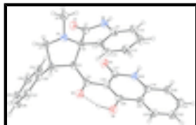
Fig. 1. The molecular structure of the title compound, showing the atomic numbering and displacement ellipsoids drawn at the 50% probability level. The dashed line indicates a hydrogen bond.
