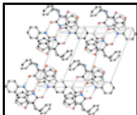
Fig. 2. The crystal packing of the title compound. H atoms not involved in hydrogen bonding (dashed lines) have been omitted for clarity.
